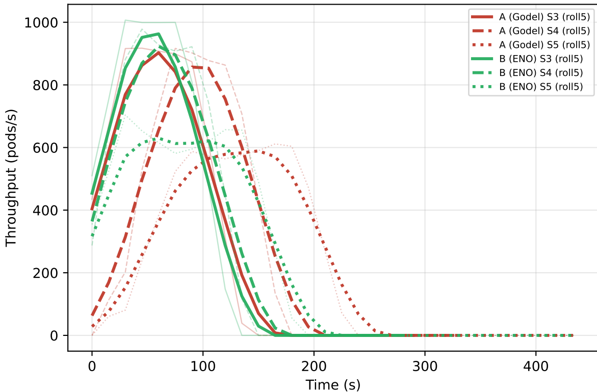
T-4 Inst3 Throughput (all points + rolling mean, no averaging) W3 Throughput (all points connected)
