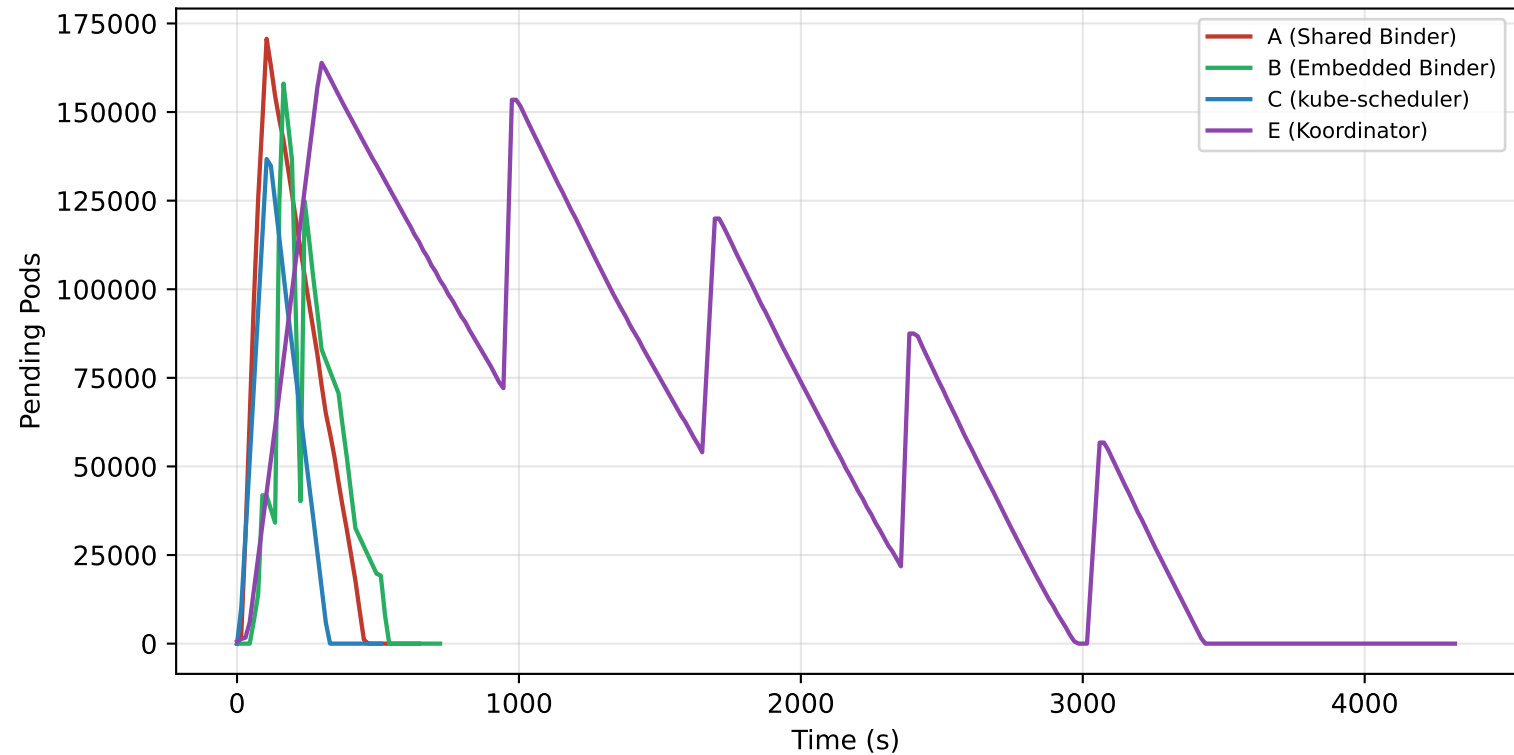
S-3 Pending Pods Time Series (W4, s3)
