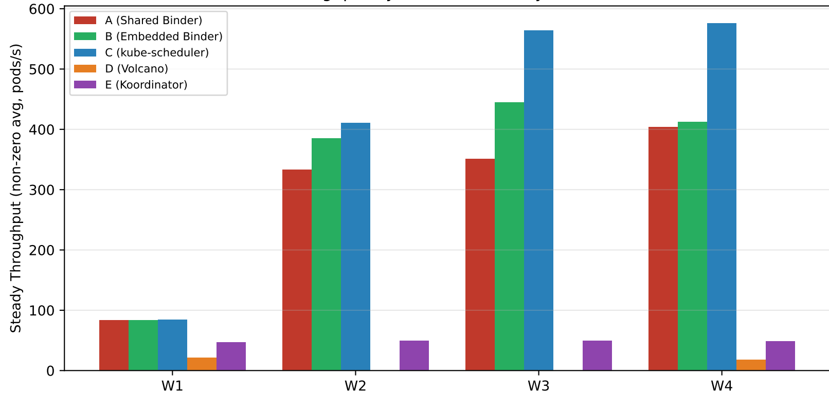
T-3 Throughput by Workload (steady, W1-W4, s3)
