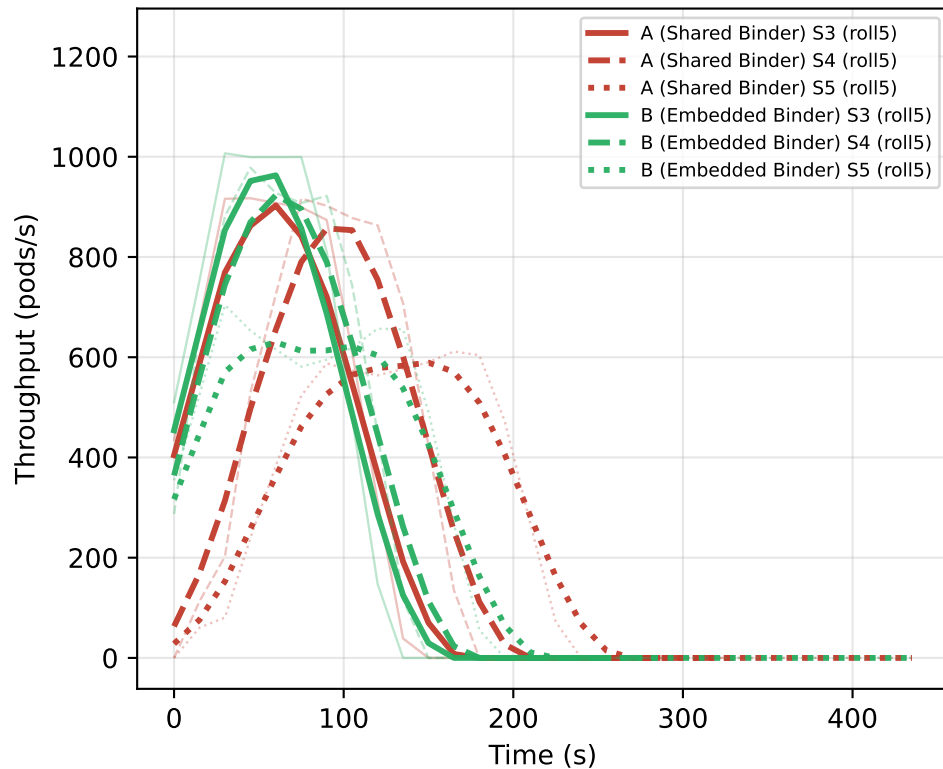
W3 Throughput (all points connected)
