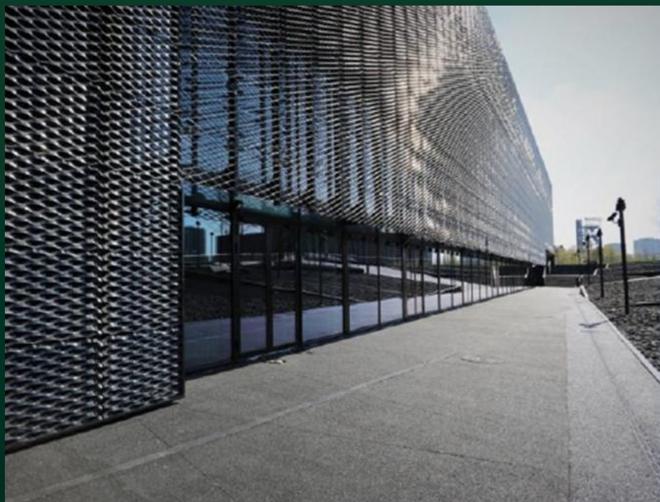
Elevation made of cut-drawn mesh (Front of House)
