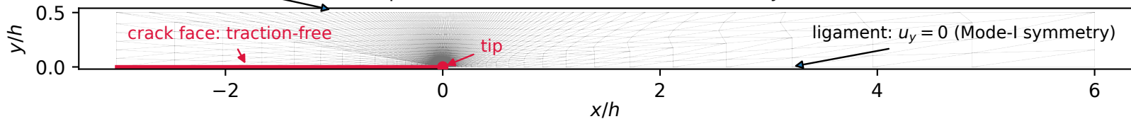
(a) strip half-model: rosette mesh and boundary conditions
