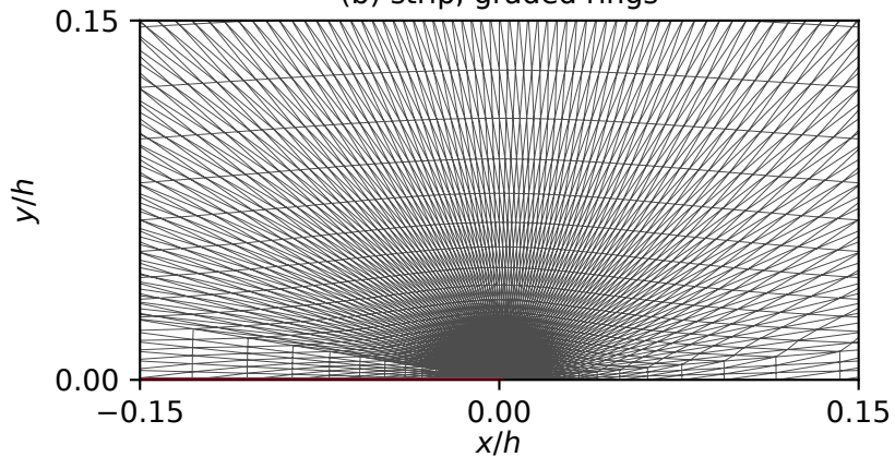
(b) strip, graded rings
