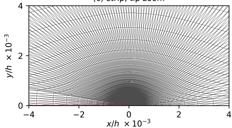
(c) strip, tip zoom
