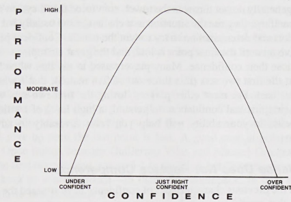
Figure 10.1 Confidence-Performance Relationship
