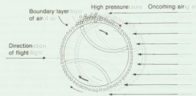
Figure 2.1: The boundary layer of air being carried around the ball in a topspin direction interacts with the oncoming air to create a high pressure zone above the ball.
