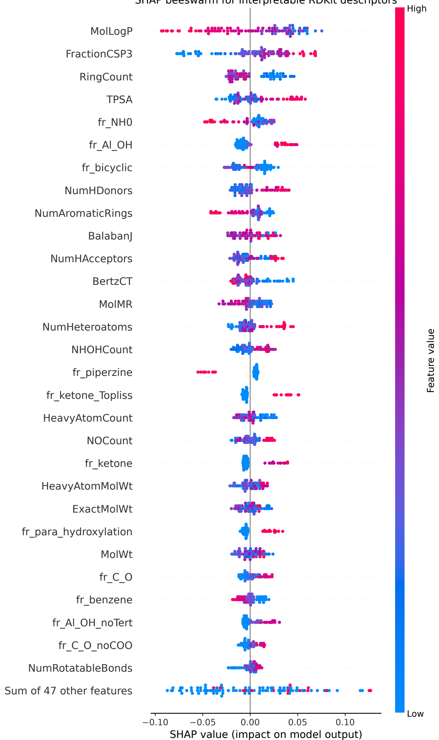
SHAP beeswarm for interpretable RDKit descriptors
