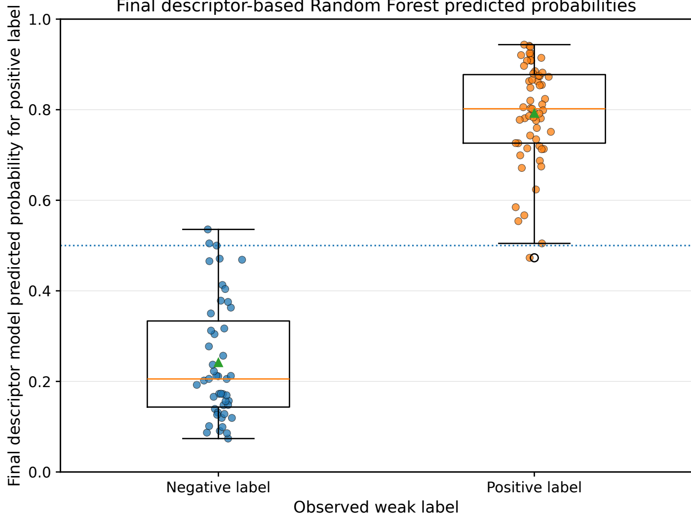
Final descriptor-based Random Forest predicted probabilities
