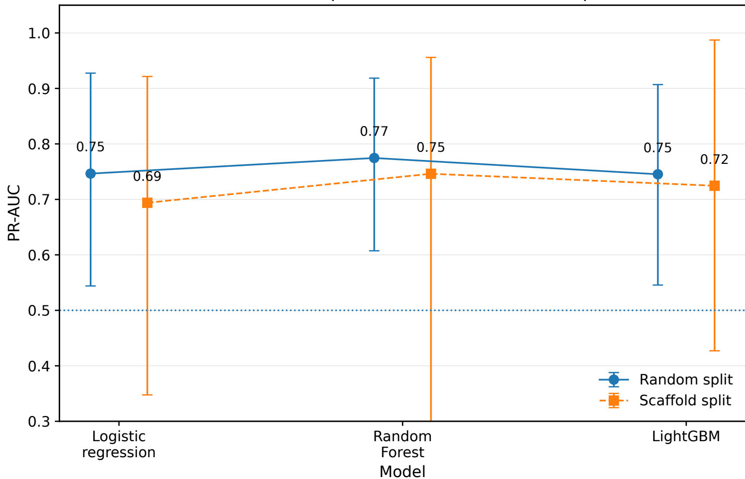
PR-AUC across repeated random and scaffold splits
