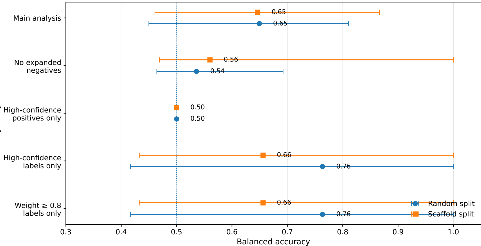
Random Forest sensitivity analysis: Balanced accuracy
