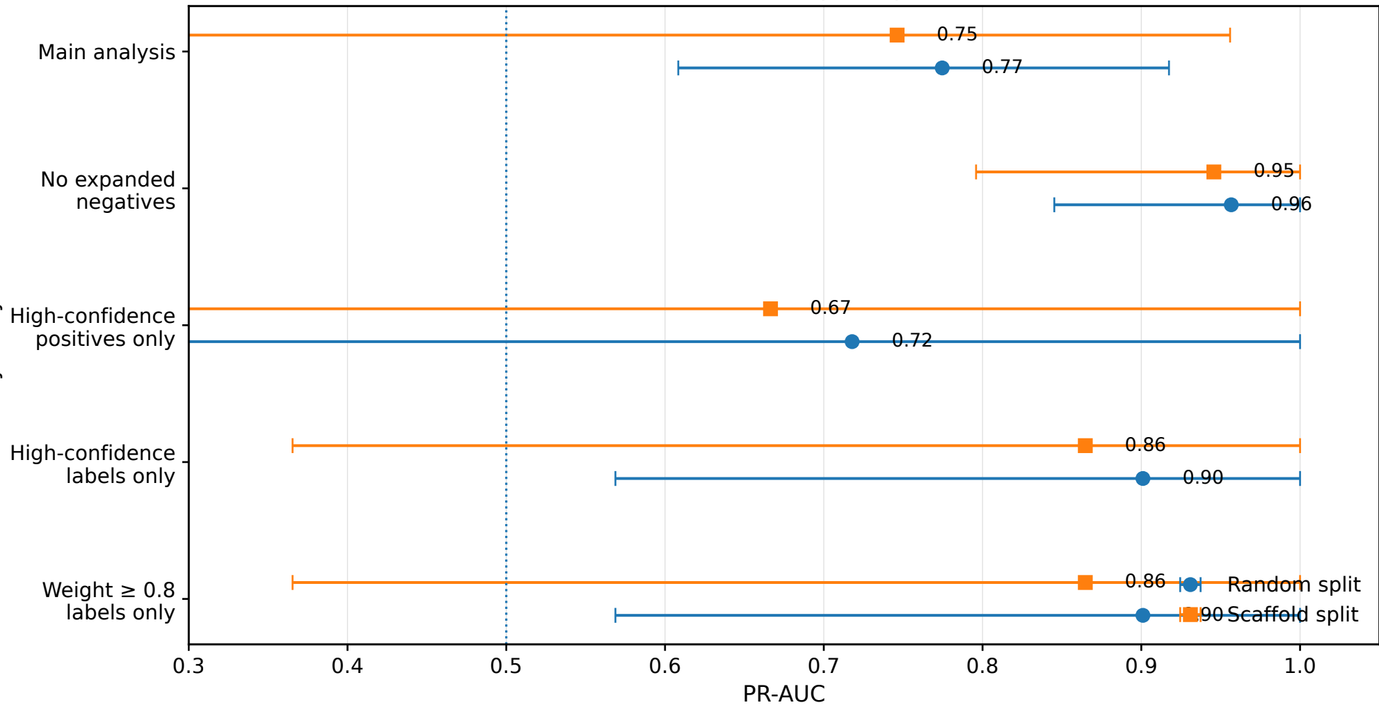
Random Forest sensitivity analysis: PR-AUC
