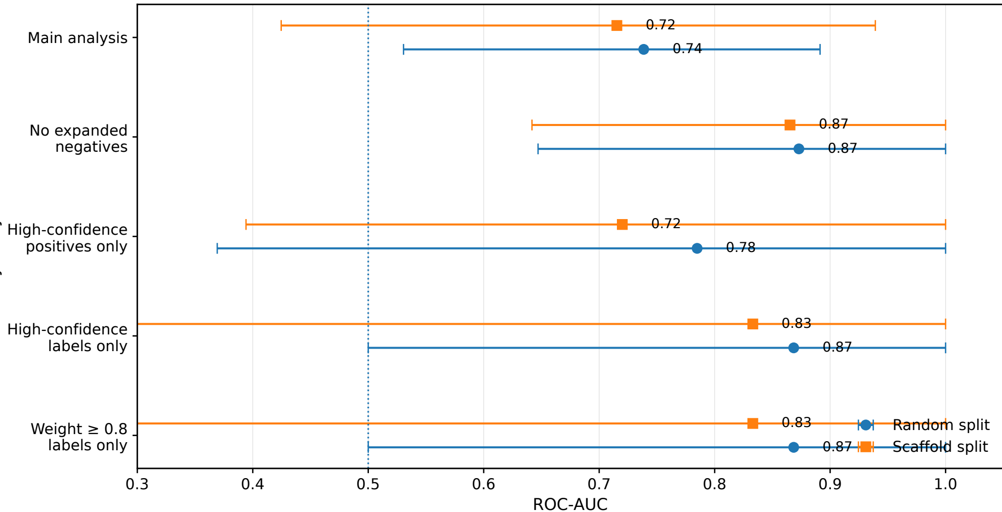
Random Forest sensitivity analysis: ROC-AUC
