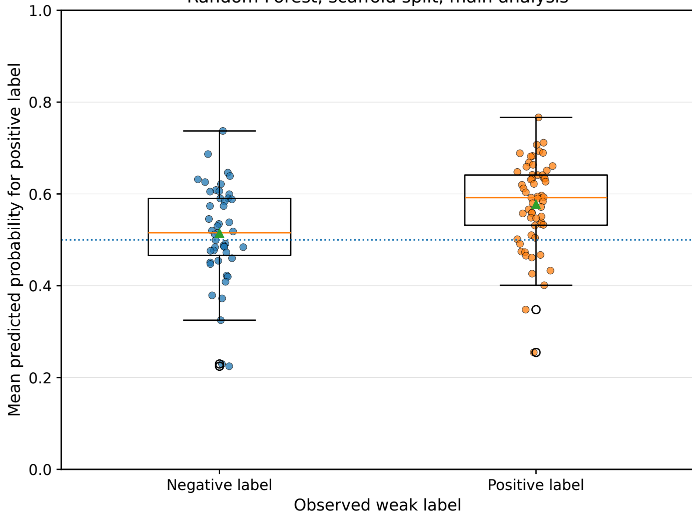
Distribution of drug-level predicted probabilities Random Forest, scaffold split, main analysis
