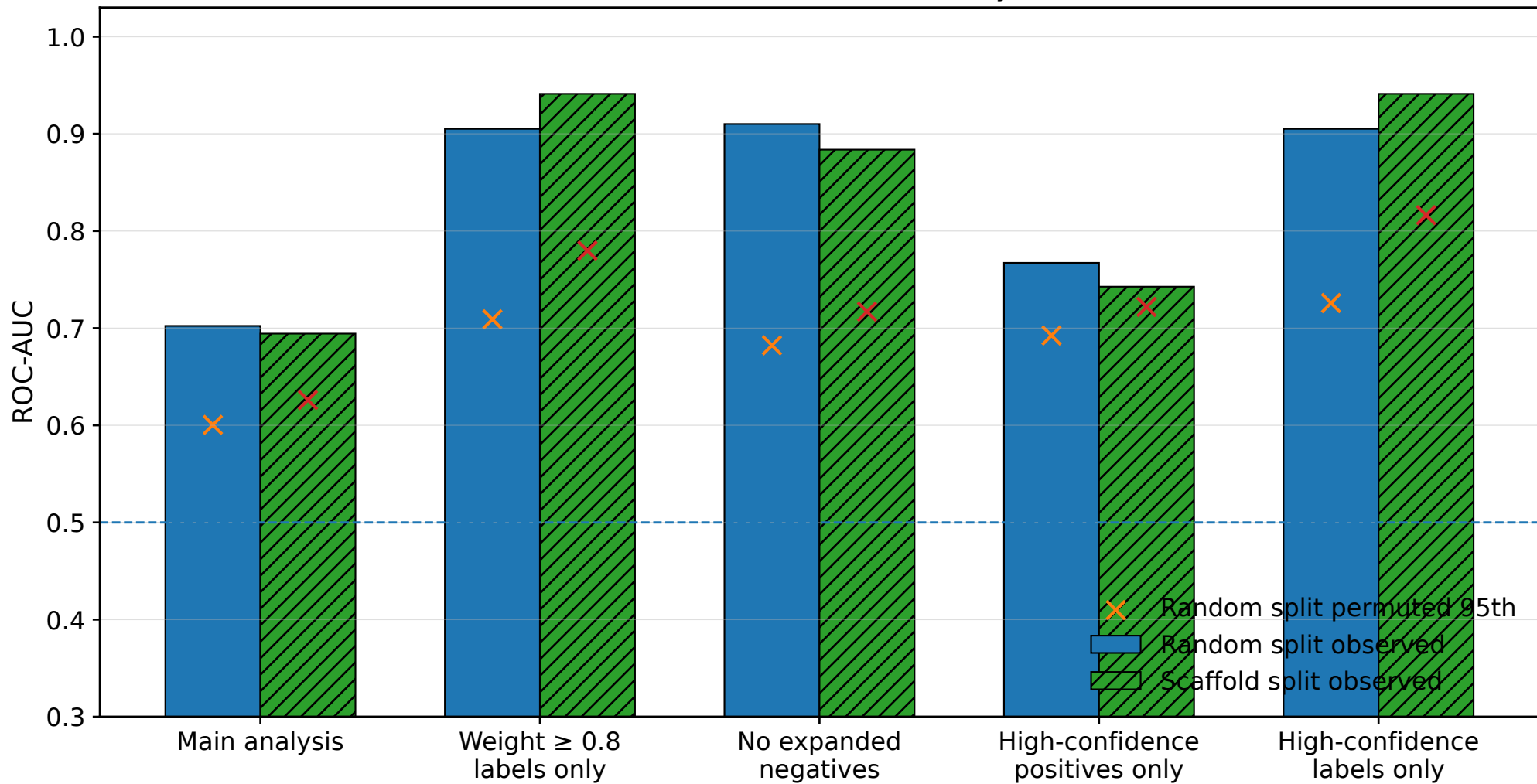
Permutation test summary
