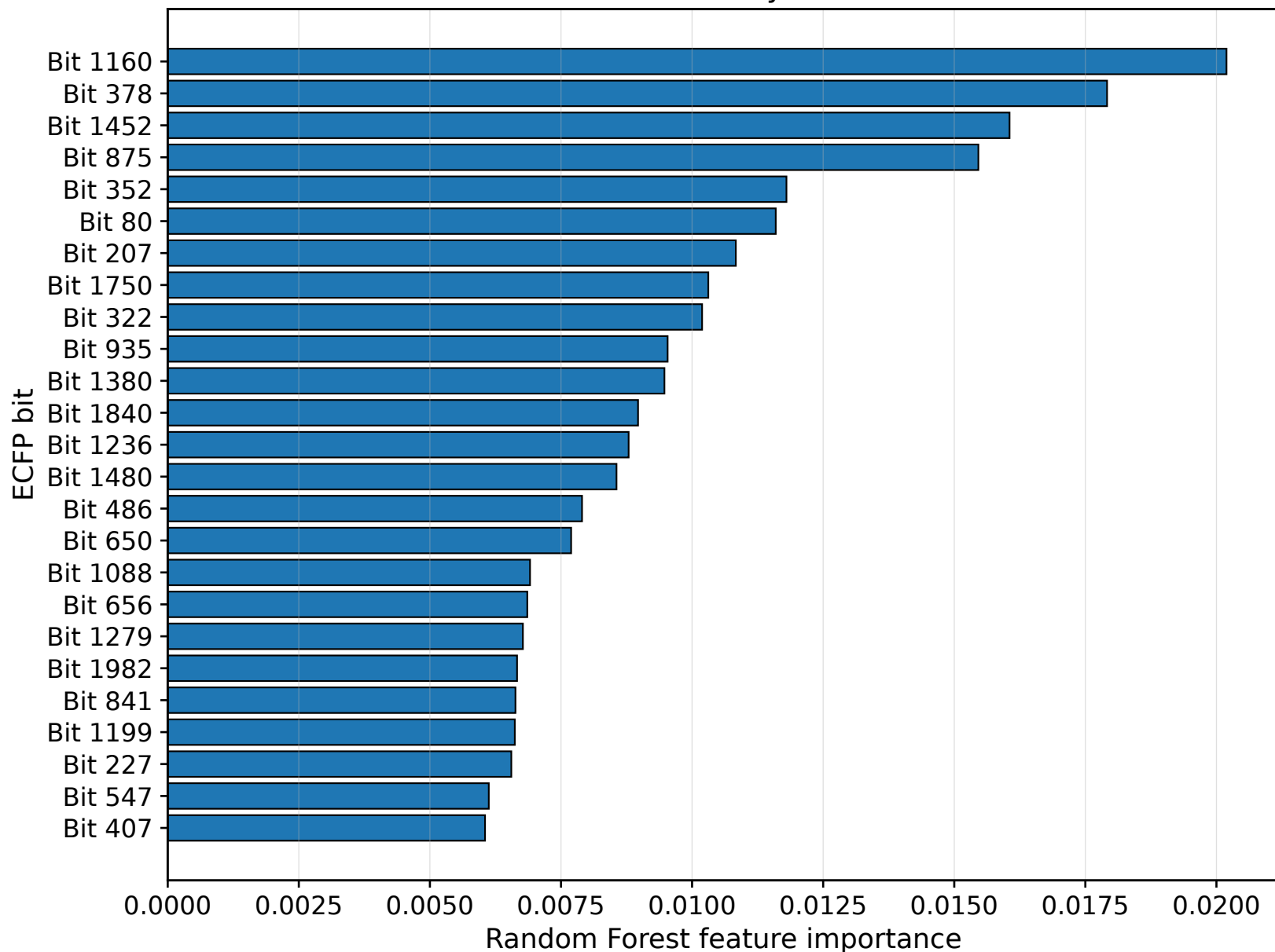
Top ECFP bits in the Random Forest model Main analysis
