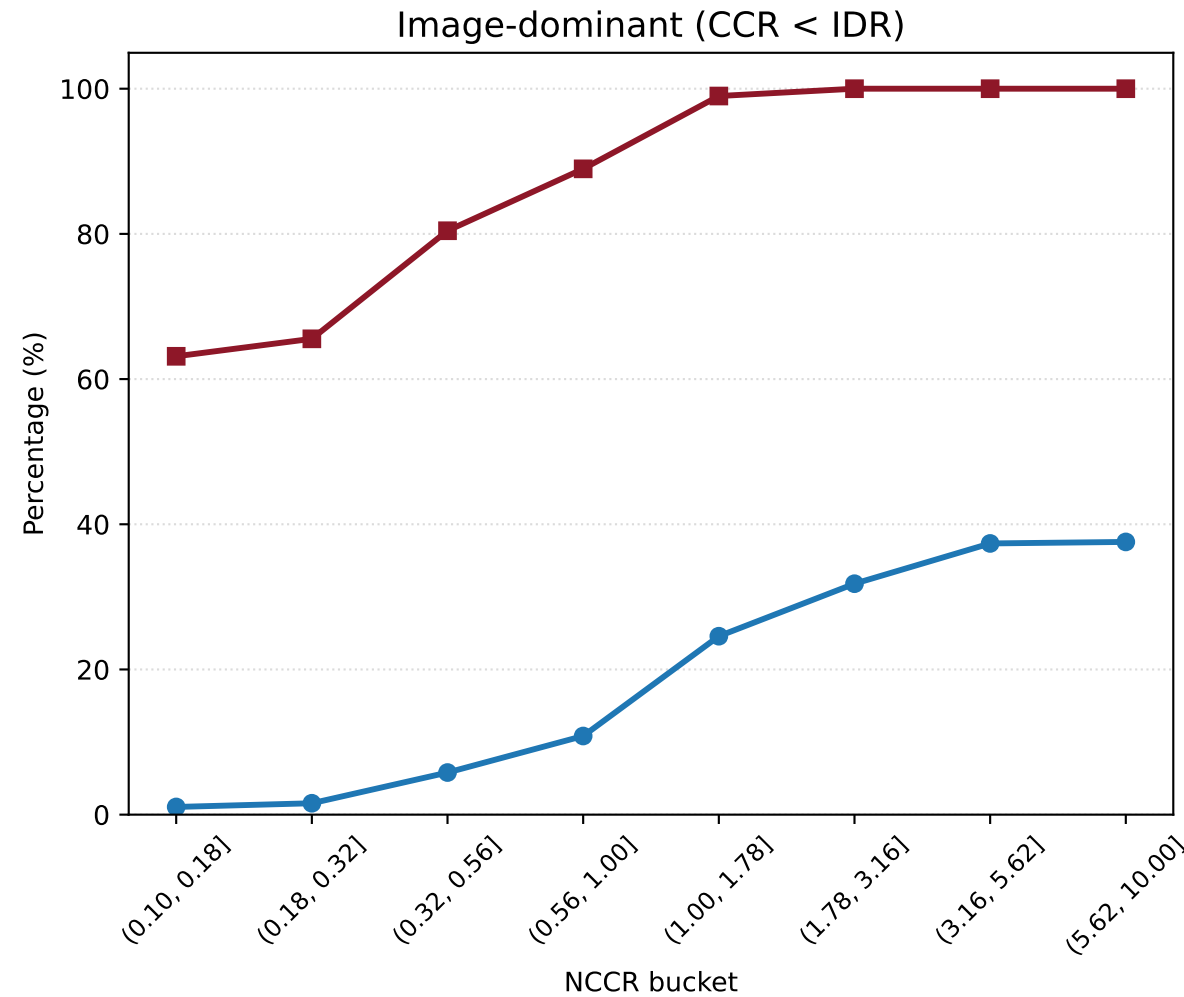
NHEFT gain rate and win rate by communication composition
