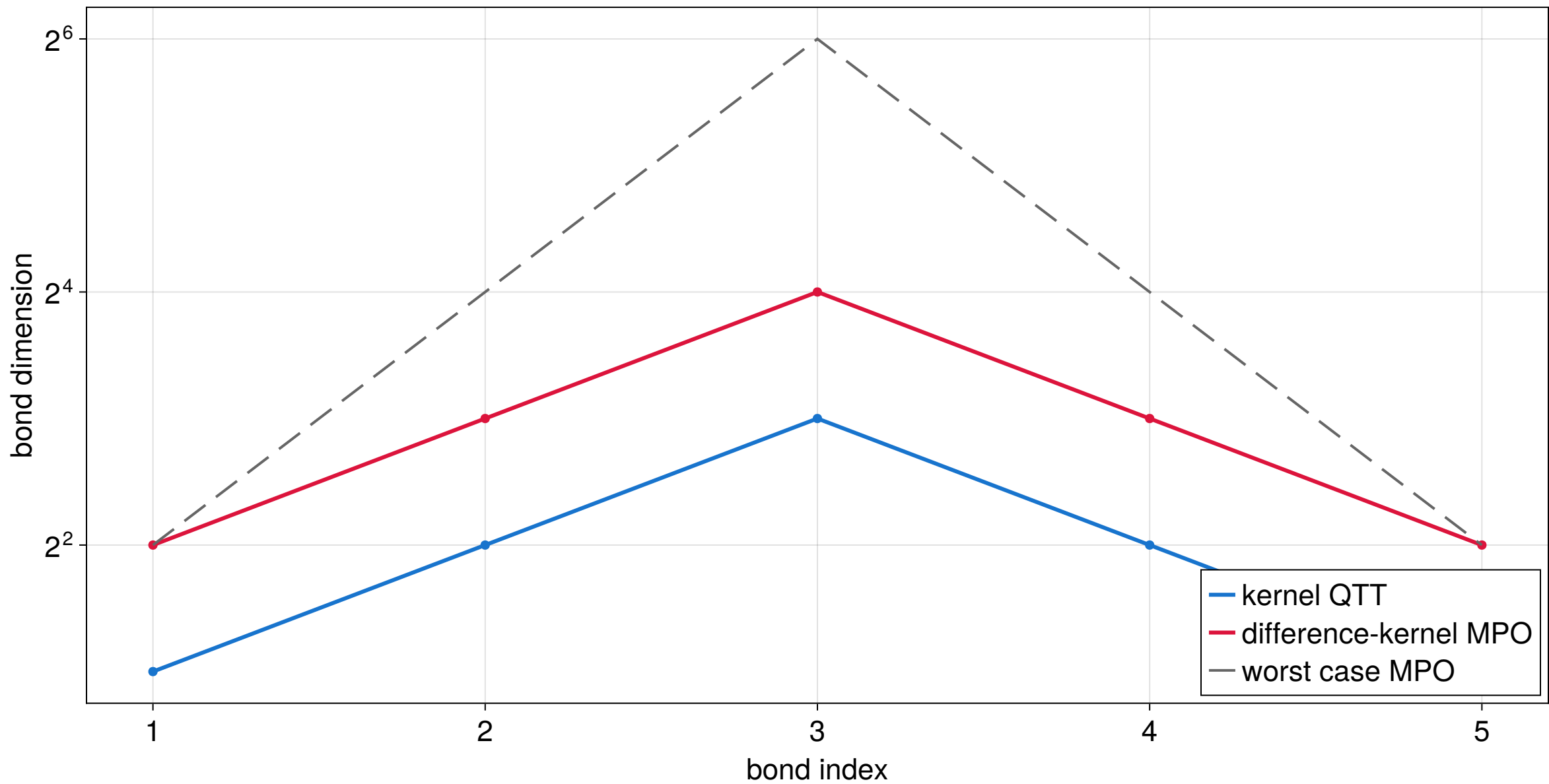
Difference-kernel MPO bond dimensions
