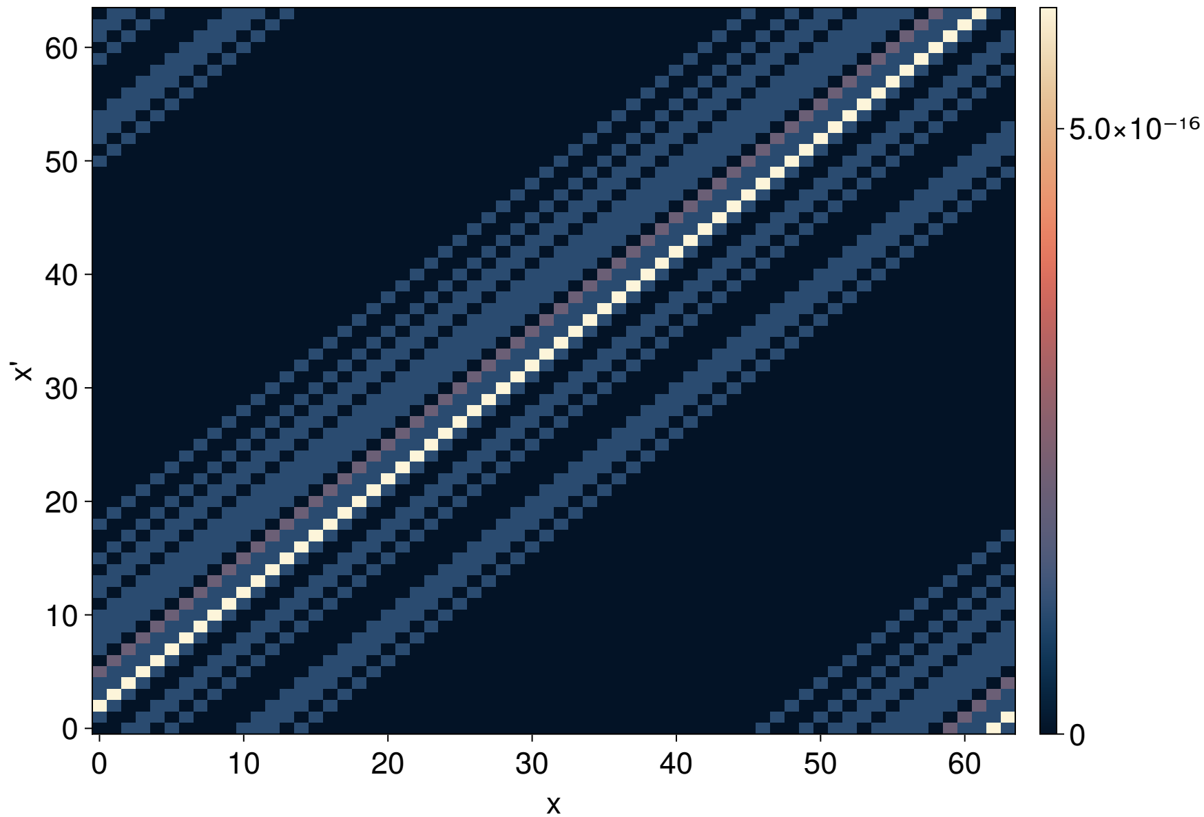
Difference-kernel MPO absolute error
