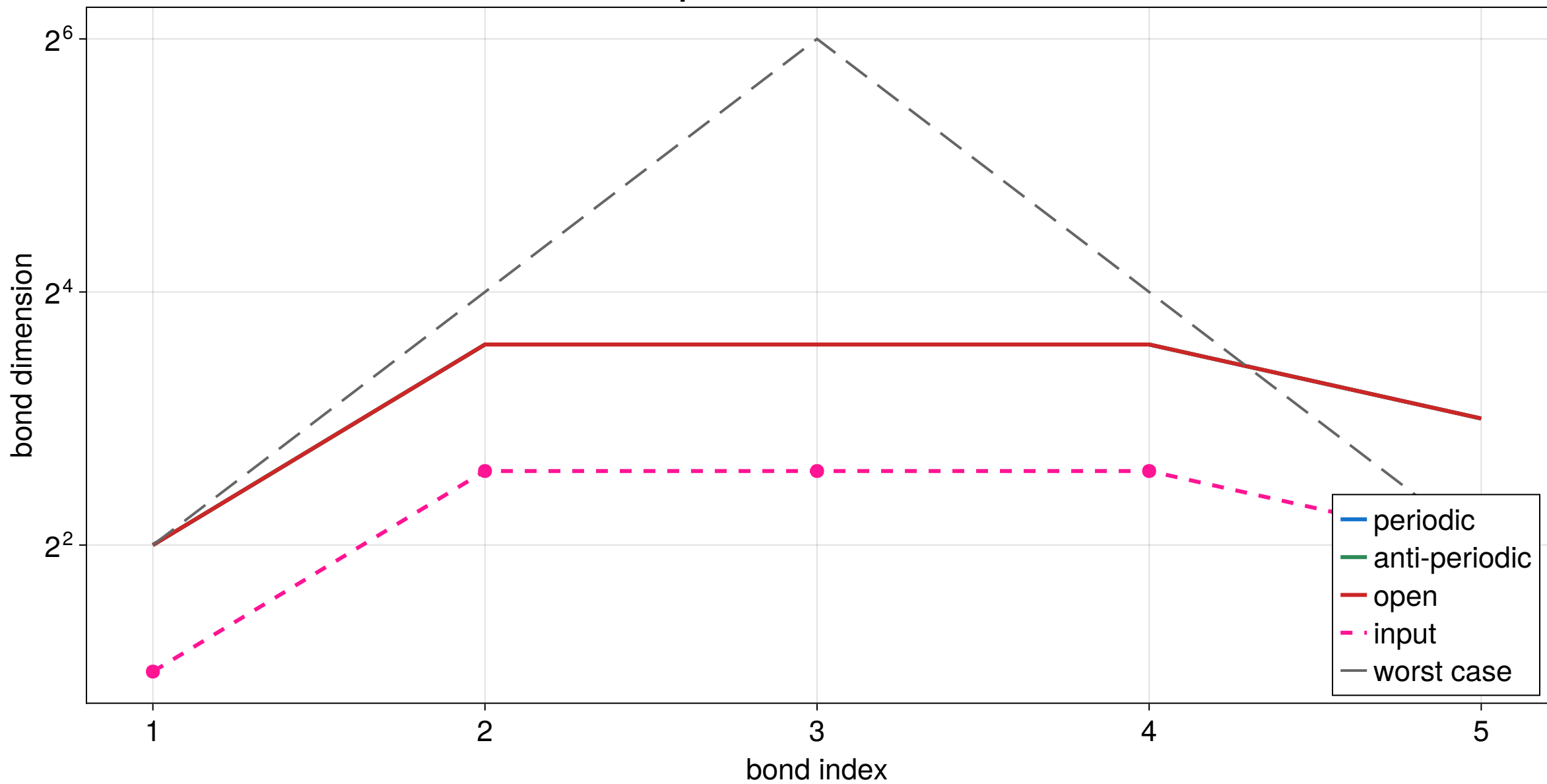
Affine pullback bond dimensions
