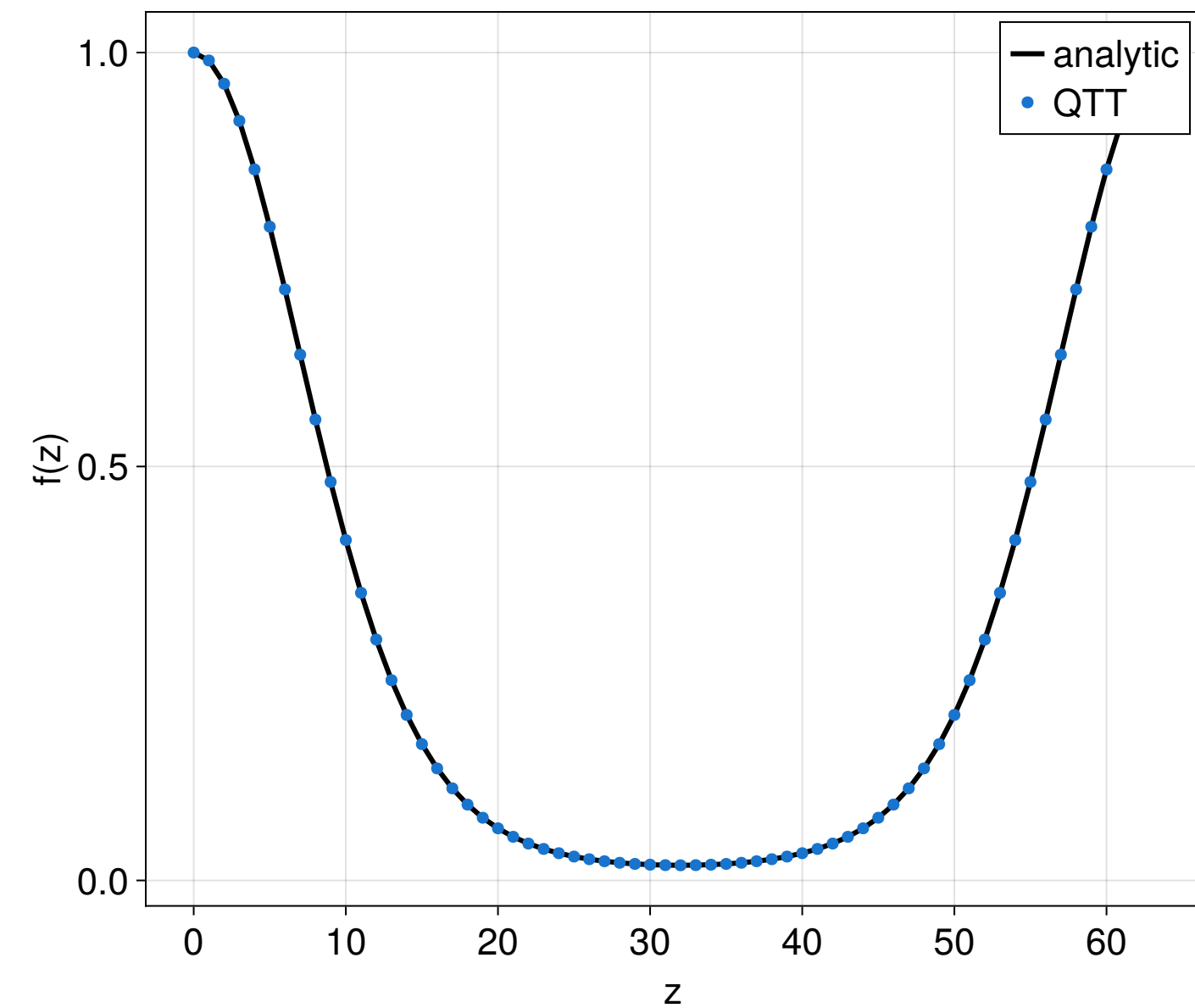
Periodic source kernel
