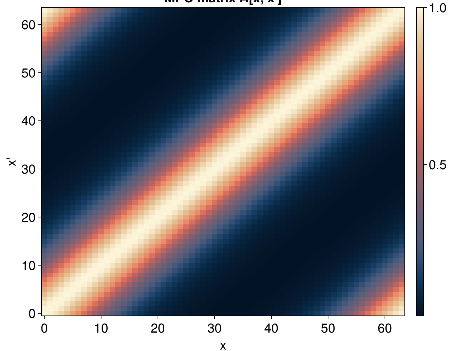
MPO matrix A[x, x']
