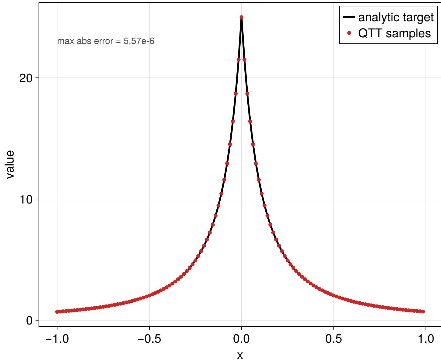
multiscale: softened 1/r^2
