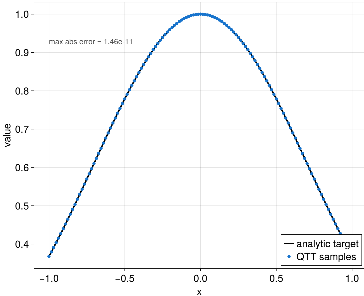
single-scale: \exp(-x^2)
