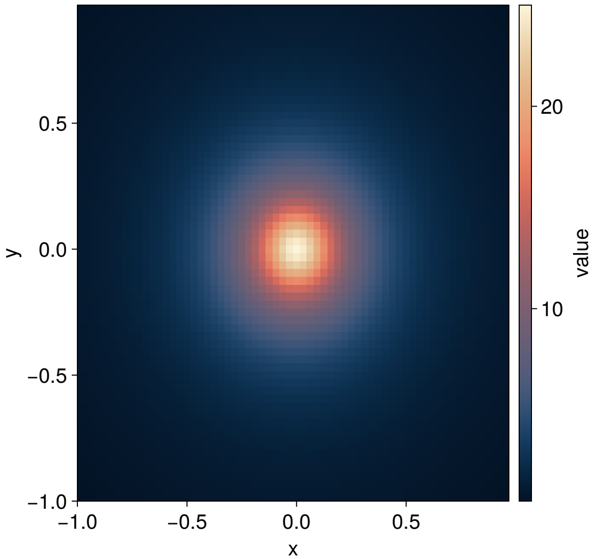
exact softened 1/r^2
