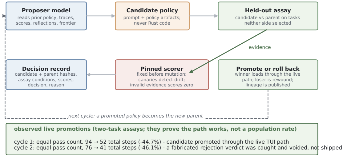
Figure 5: Policy-level self-improvement. The proposer never grades its candidate; a pinned scorer decides on held-out evidence, and every decision is recorded with the hashes and conditions that produced it.
