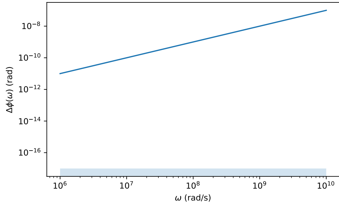
FIGURE S2: Causal phase shift \Delta\phi(\omega)
