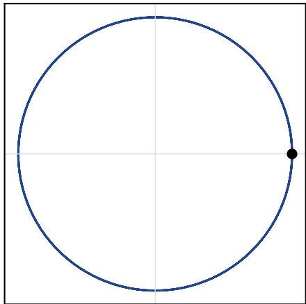
\sigma = 1/2 : closed loop
