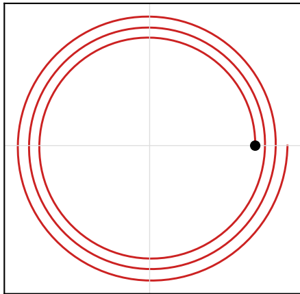
\sigma = 0.7 : outward spiral
