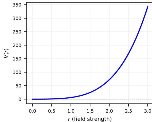
Mixed S_{02}
