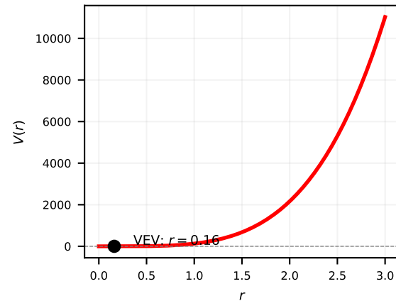
Best Sombbrero
