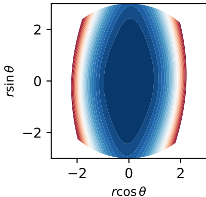
\Delta\mathcal{I} Landscape (Mexican Hat)
