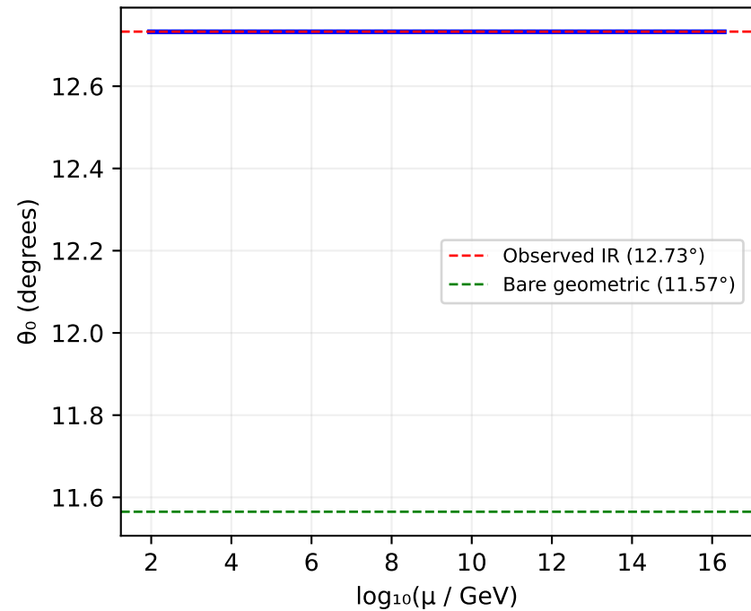
Koide Angle RG Flow
