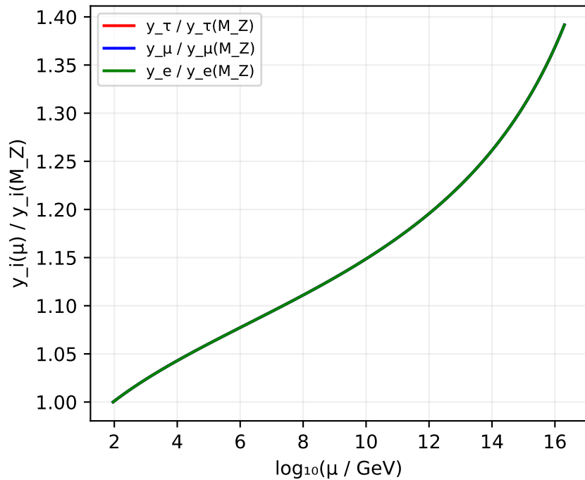
Yukawa Coupling Running
