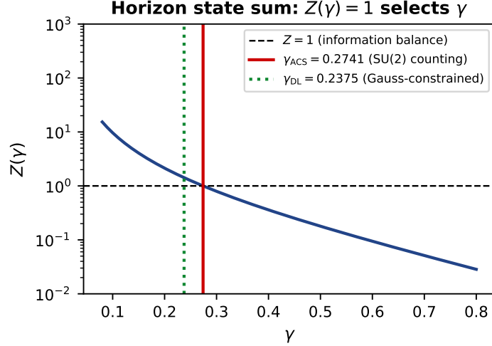
Figure 9: The partition function Z(\gamma) = \sum_j (2j+1) e^{-2\pi\gamma\sqrt{j(j+1)}} . The ACS information balance condition Z = 1 (dashed) selects \gamma_{\text{ACS}} = 0.274 (red). The Domagala–Lewandowski value \gamma \approx 0.238 (green, dotted) uses a more restrictive counting that excludes integer- j contributions via the horizon U(1) projection constraint. The 15% gap is the quantitative signature of this boundary condition.
