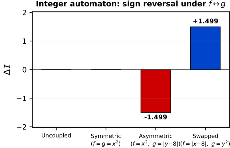
Figure 4: Sign reversal of \Delta\mathcal{I} under f \leftrightarrow g swap. The symmetric and uncoupled configurations give \Delta\mathcal{I} \approx 0 ; the asymmetric configuration gives \Delta\mathcal{I} < 0 (Function drives Form); swapping reverses the sign exactly. Computed in exact integer arithmetic on \mathbb{Z}_{16} .
