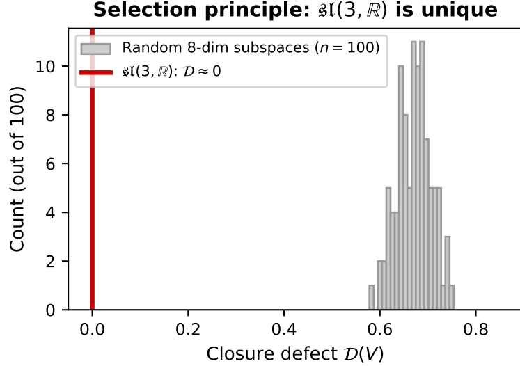
Figure 5: The closure defect \mathcal{D}(V) for 100 randomly sampled 8-dimensional subspaces of \mathfrak{sl}(4, \mathbb{R}) (grey histogram), compared with \mathfrak{sl}(3, \mathbb{R}) at \mathcal{D} = 0 (red line). No random subspace achieves \mathcal{D} < 0.54 ; the subalgebra \mathfrak{sl}(3, \mathbb{R}) is the unique closure attractor.
