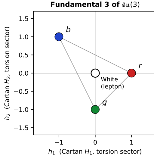
Figure 6: Weight diagram of the fundamental 3 representation of \mathfrak{su}(3) . The three colour charges are the eigenvalues of the Cartan generators H_1 , H_2 , both of which sit in the torsion sector of the Palatini decomposition. The colourless (lepton) state at the origin has zero eigenvalue under both generators.
