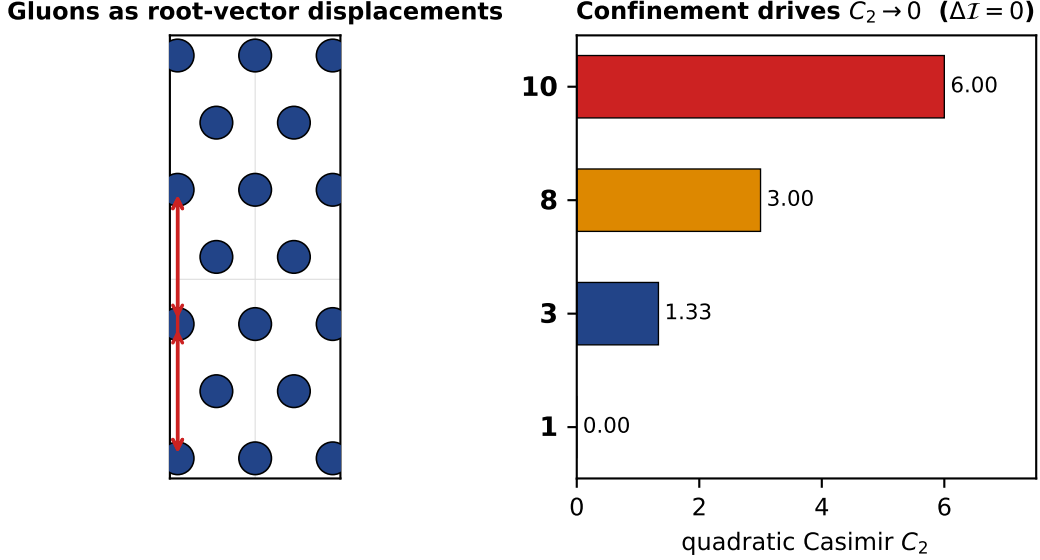
Figure 7: Left: gluon exchange as root vector displacements in the colour weight space. Each arrow represents a gluon mediating a colour rotation; the three pairs (\alpha_1, \alpha_2, \alpha_1 + \alpha_2) correspond to the three torsion–Lorentz gluon pairs. Right: representations stacked by quadratic Casimir C_2 (binding energy scale). Confinement drives the system from higher representations toward the singlet ( C_2 = 0 , \Delta I = 0 ).
