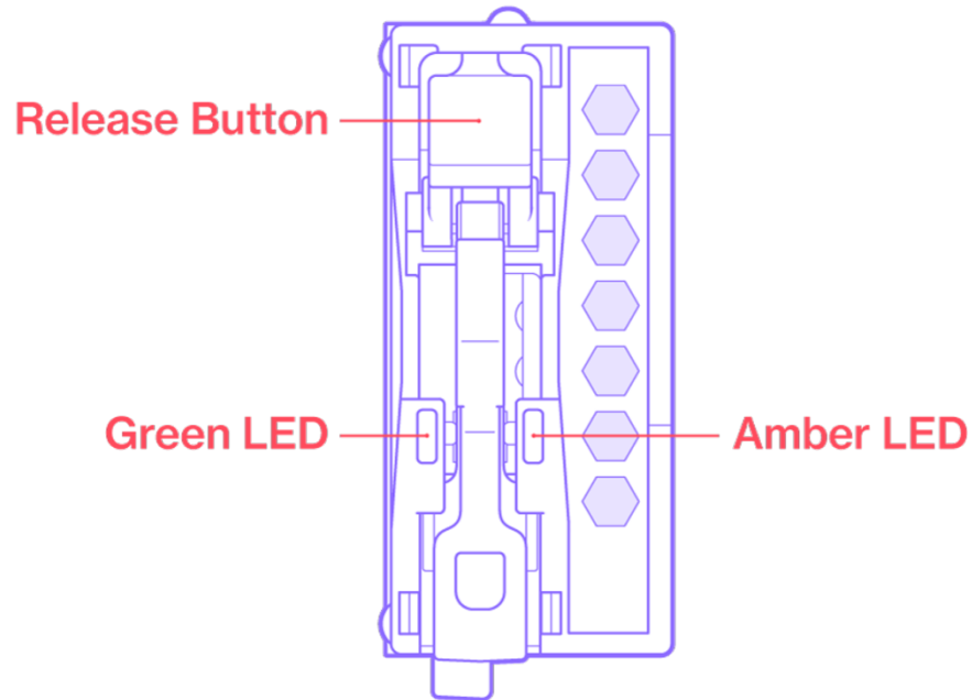
Figure 7 E1.S Overview
