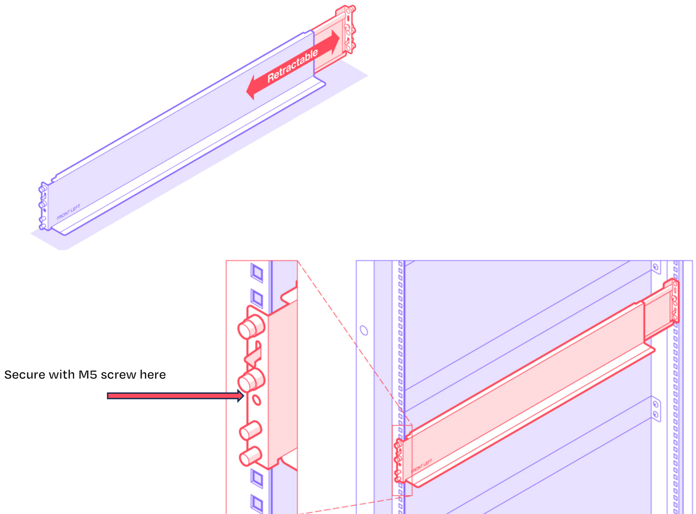
Figure 12 Illustration of Rack Assembly
