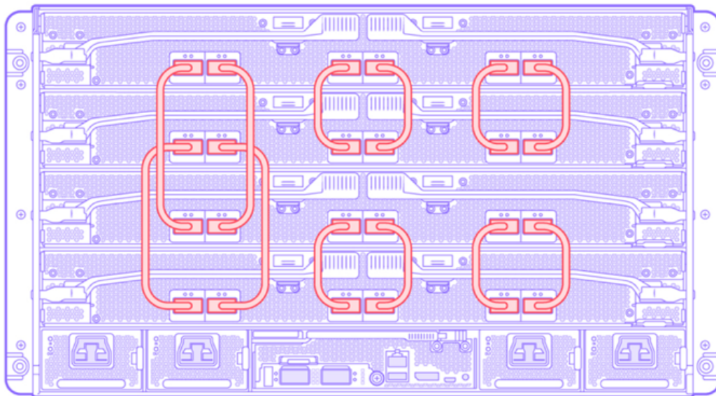
Figure 1 Diagram of Default Single Server Cable Routing
