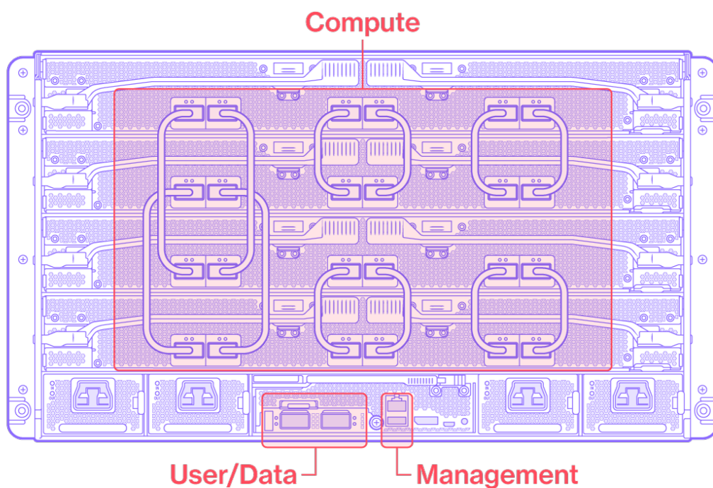
Figure 2 Highlight of Networking Areas
