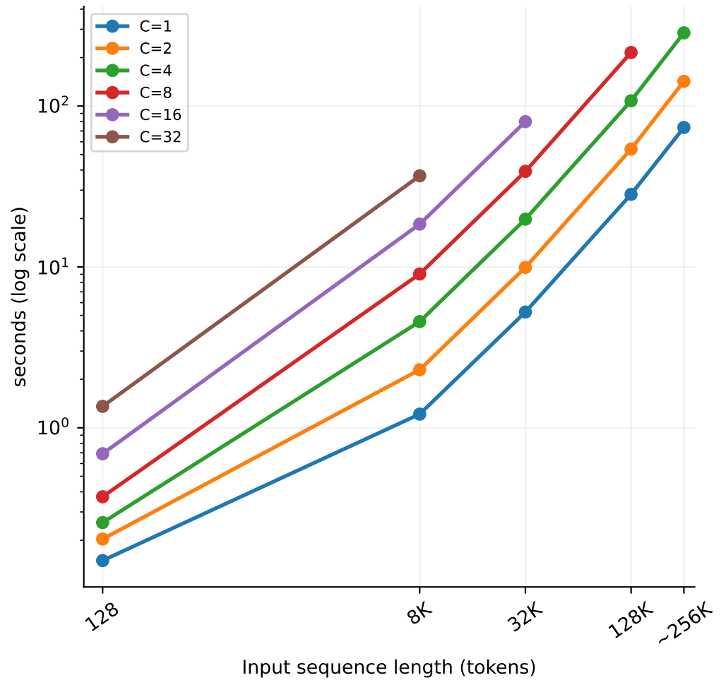
Time to first token
