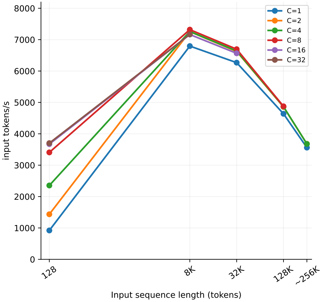
Aggregate input / prefill throughput
