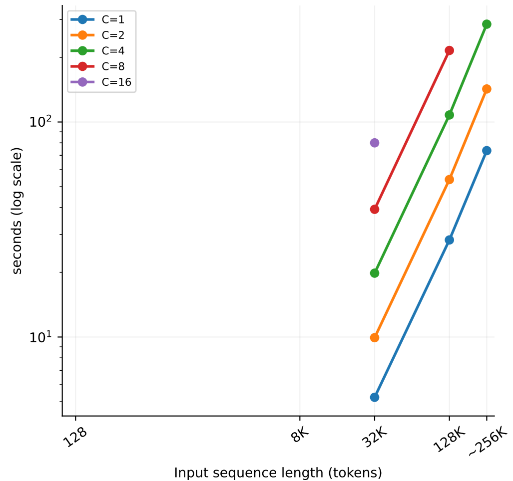
Time to first token
