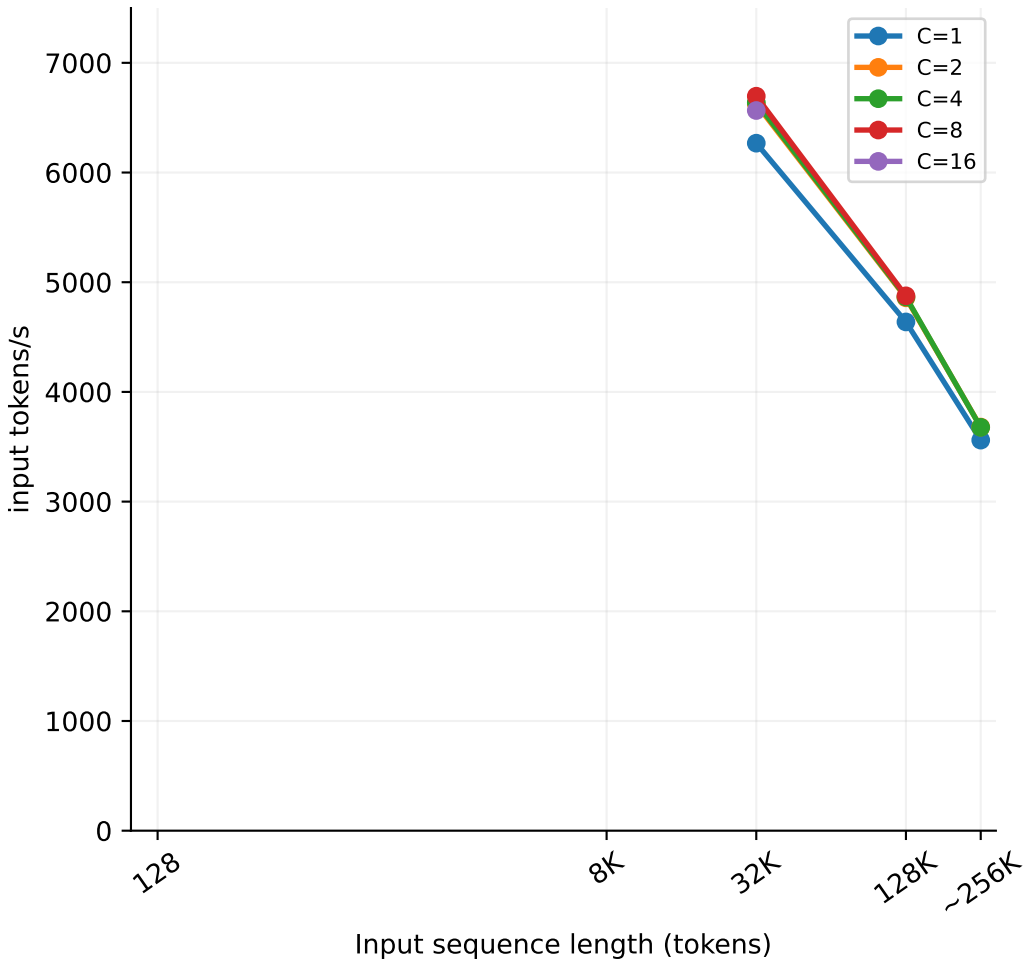
Aggregate input / prefill throughput
