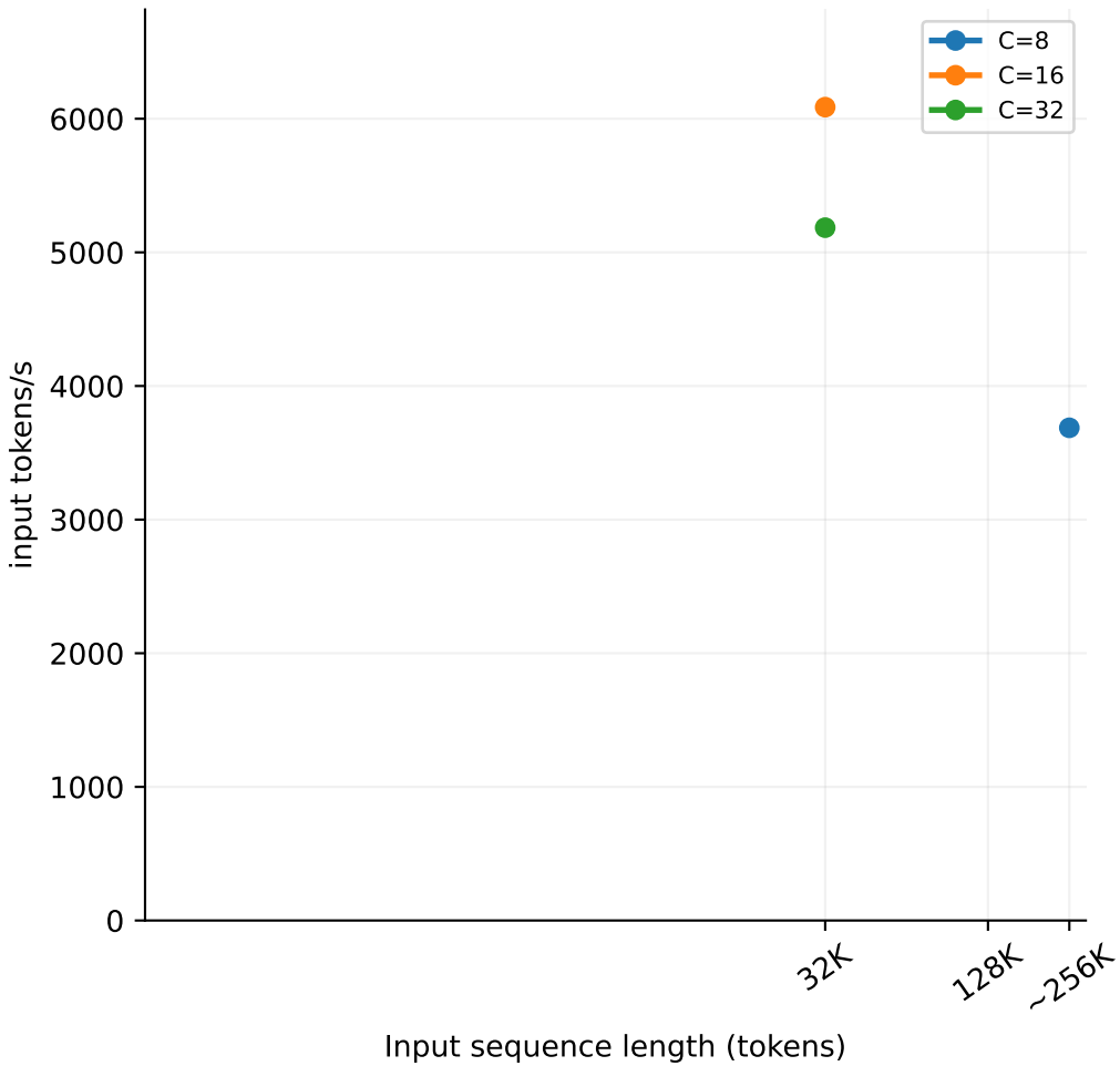
Aggregate input / prefill throughput
