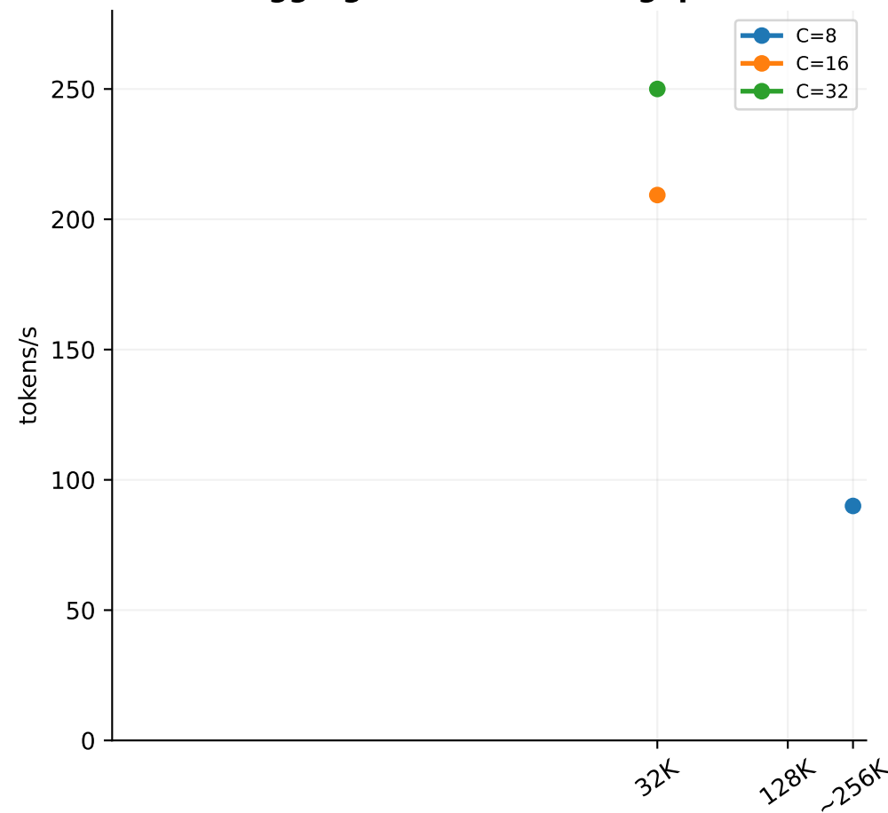
Aggregate decode throughput
