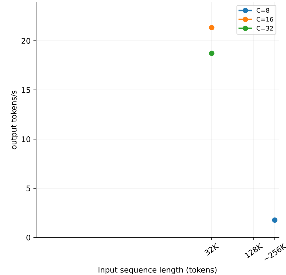
Output throughput over entire request
