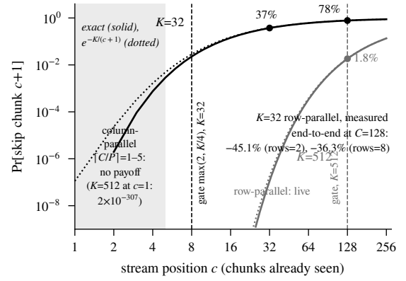
Fig. 2. Skip law (Eq. 2, model curves); the only silicon numbers are the annotated end-to-end deltas.
