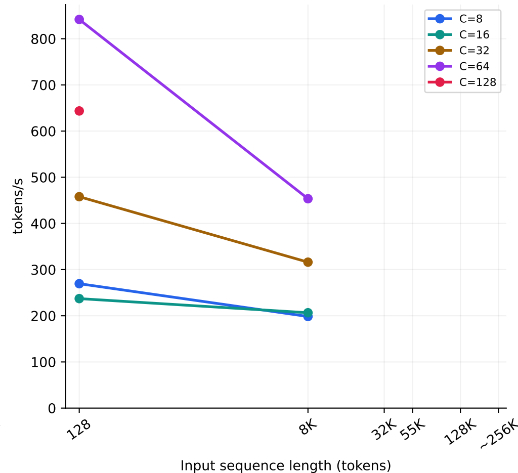
Aggregate end-to-end throughput
