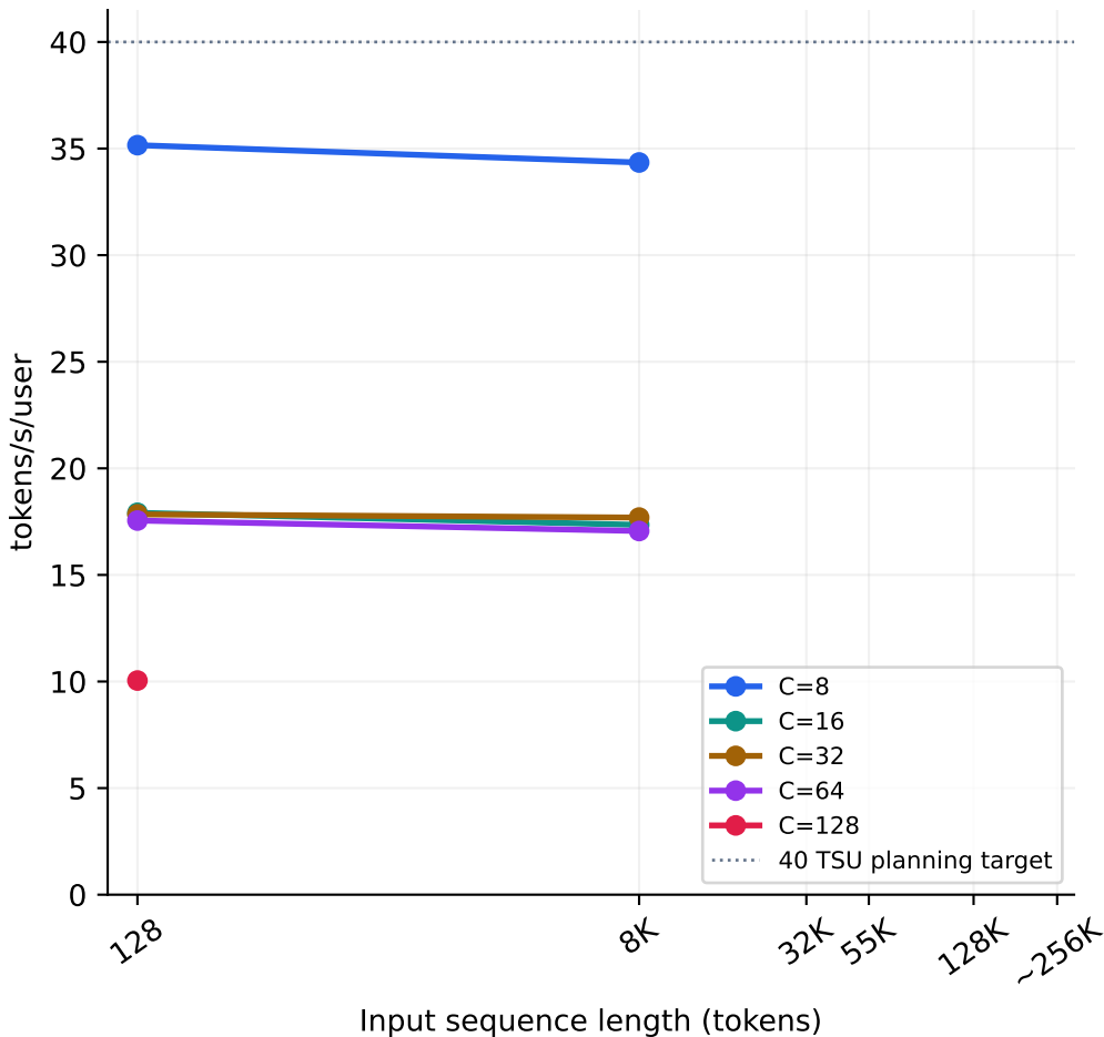
Median client decode speed
