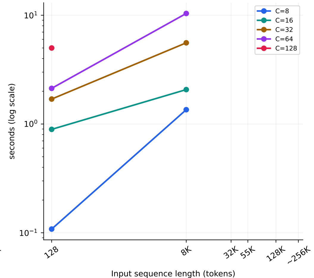
Time to first token
