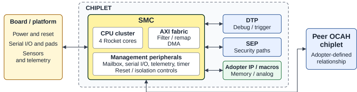
Dashed boundary: one chiplet. Clocks, macros, Boot ROM, address map and management policy are adopter-defined.
