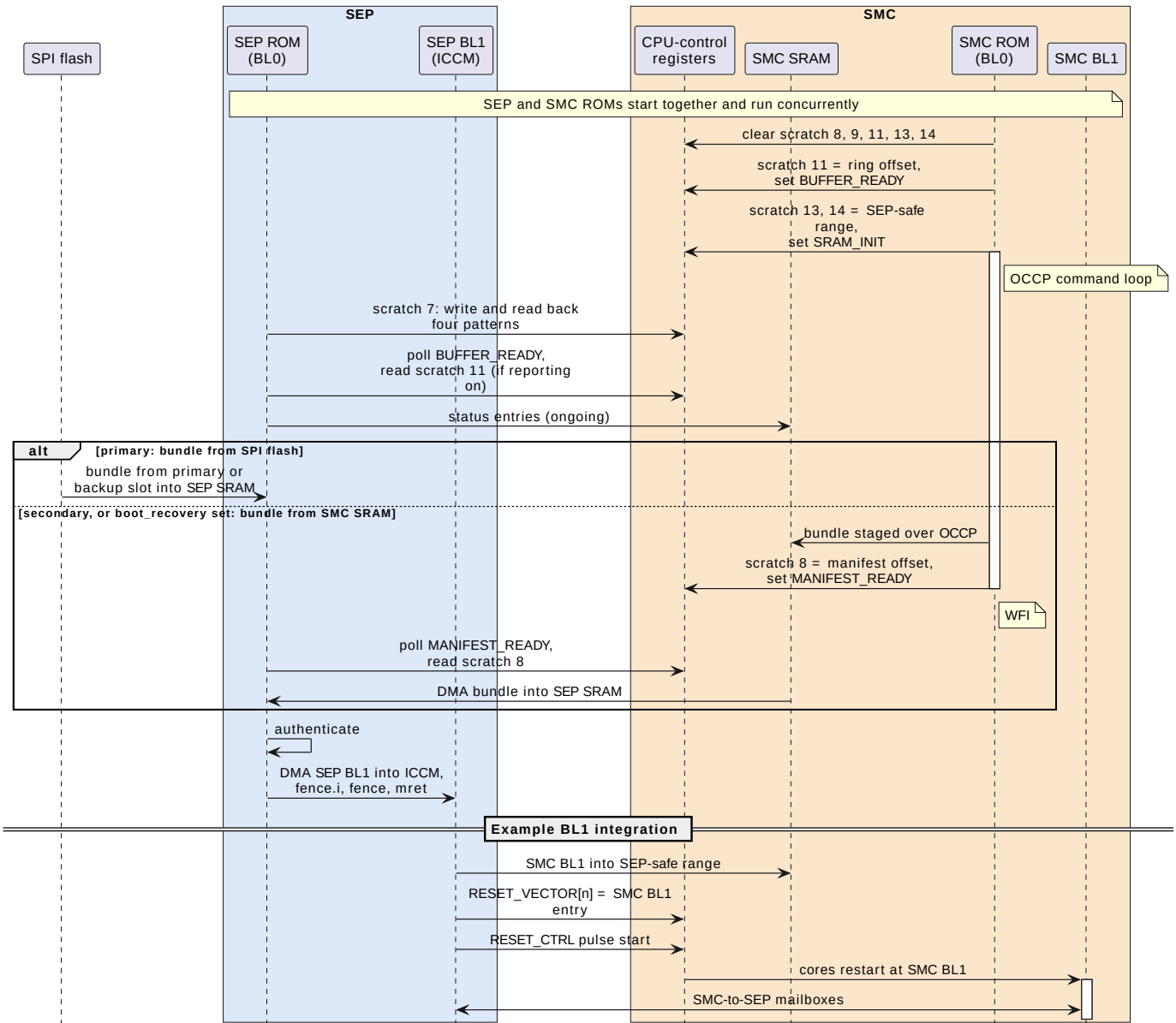
Figure 2. SEP-to-SMC coordination on one chiplet
