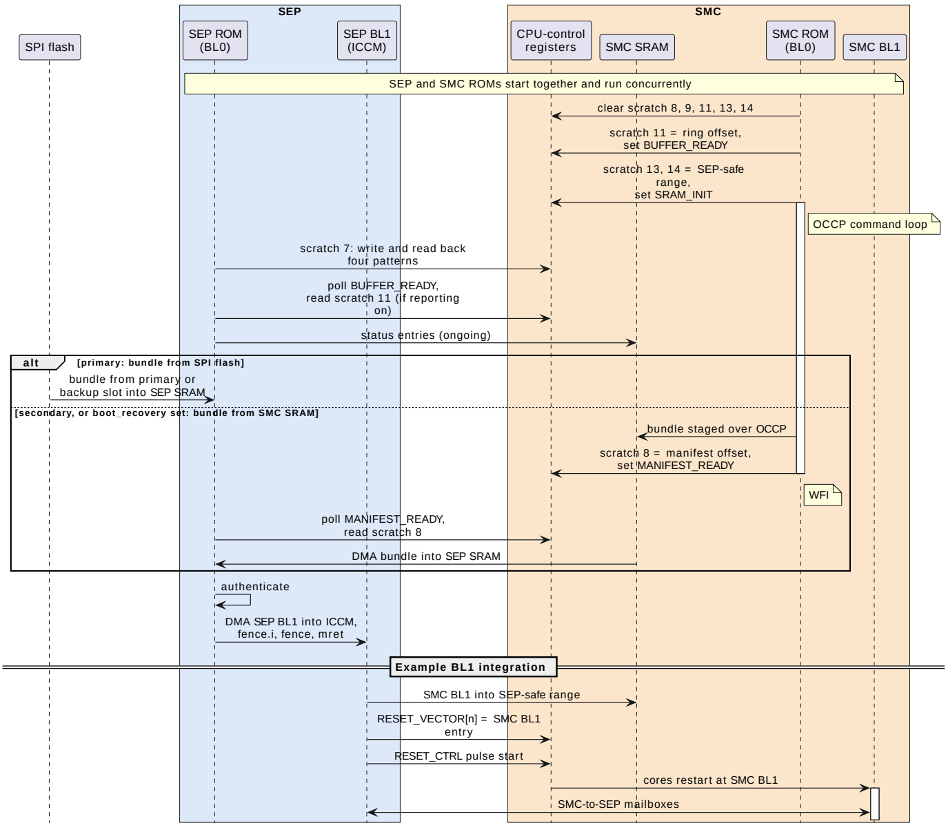
Figure 2. SEP-to-SMC coordination on one chiplet
