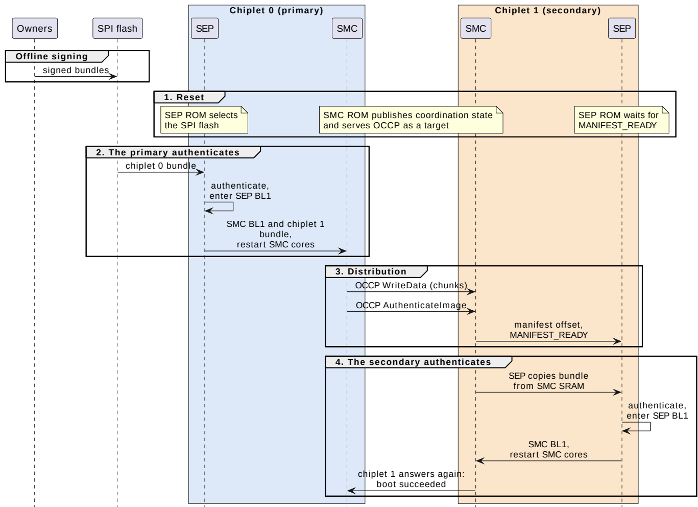
Figure 1. Package boot overview
