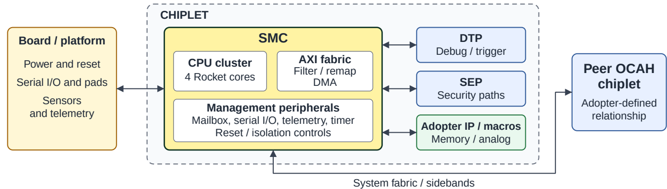
Dashed boundary: one chiplet. Clocks, macros, Boot ROM, address map and management policy are adopter-defined.
