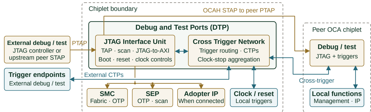
Adopter supplies pads, policy, clocks, resets, scan chains and permitted mappings.
