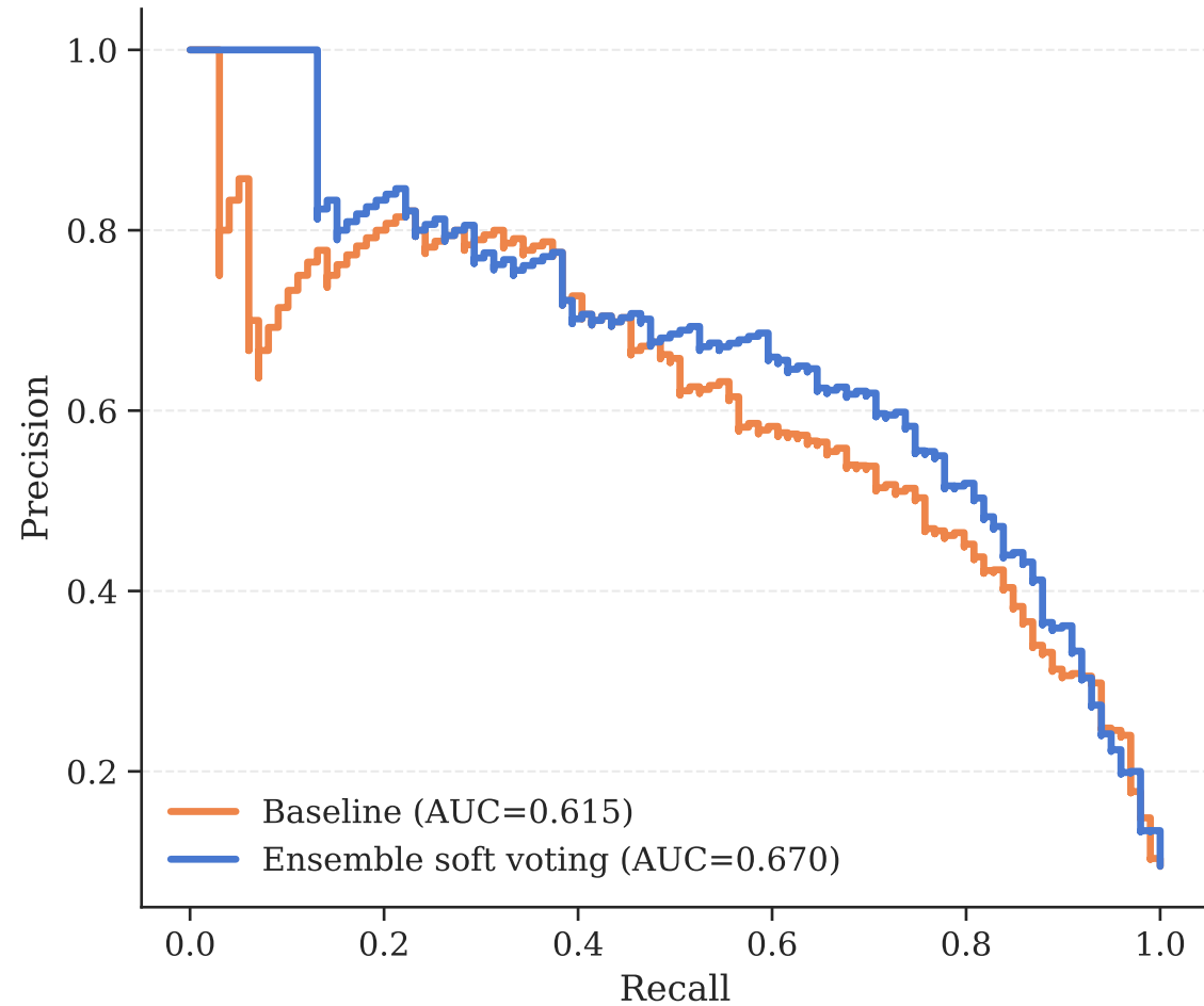
(a) Precision-Recall Comparison
