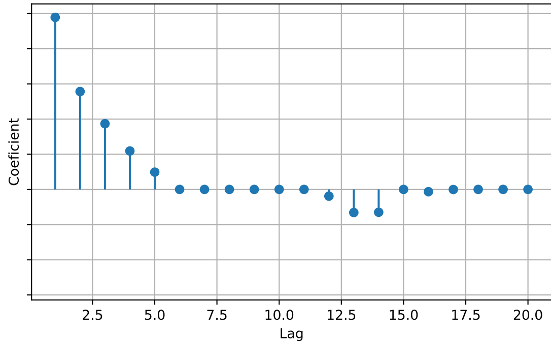
AR sparse - CVXOPT l1
