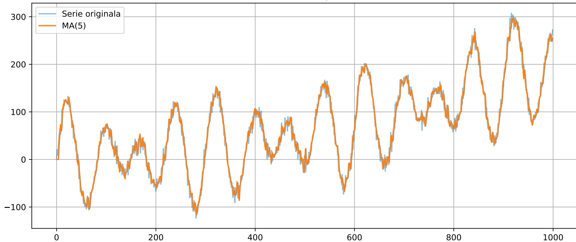
Model MA(p)
