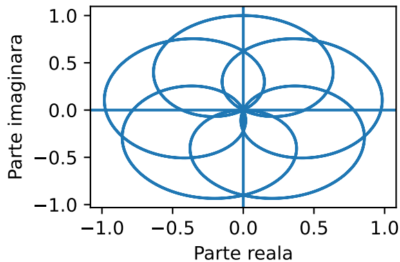
\Omega = 7
