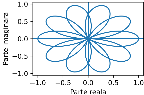
\Omega = 2
