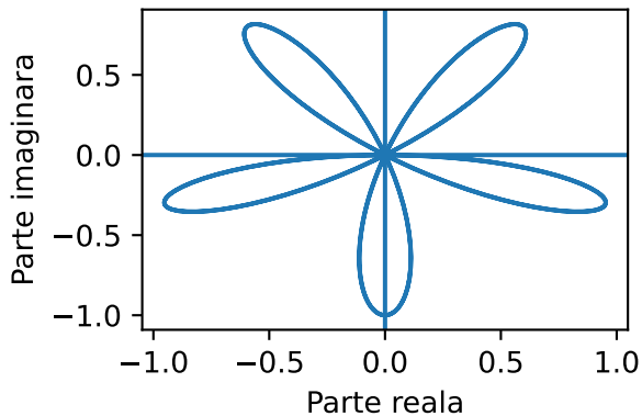
\Omega = 1
