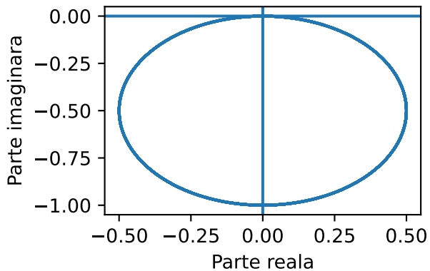
\Omega = 5
