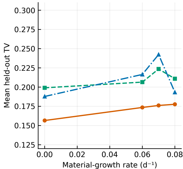
Asymmetric binary
