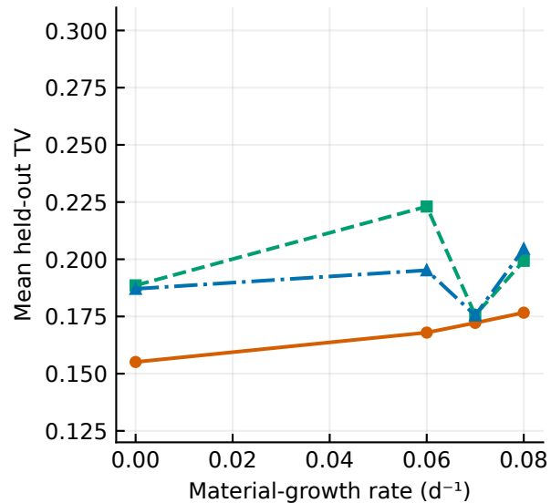
Broad binary
