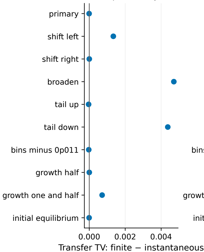
Equal binary
