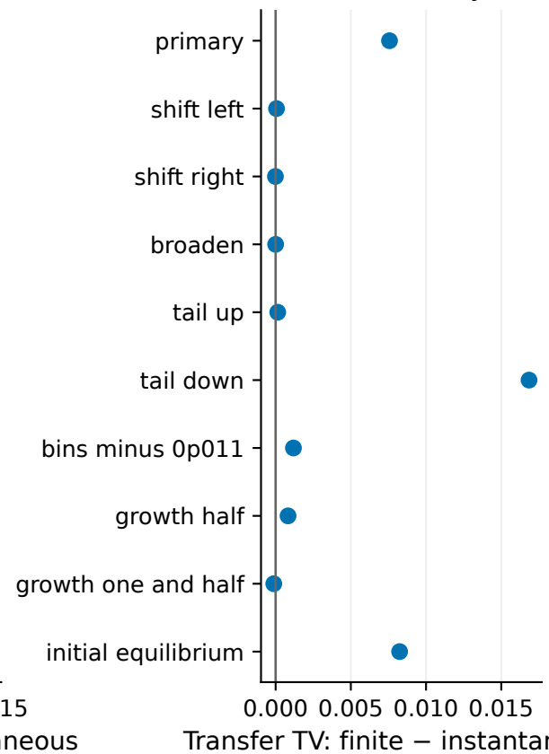
Broad binary
