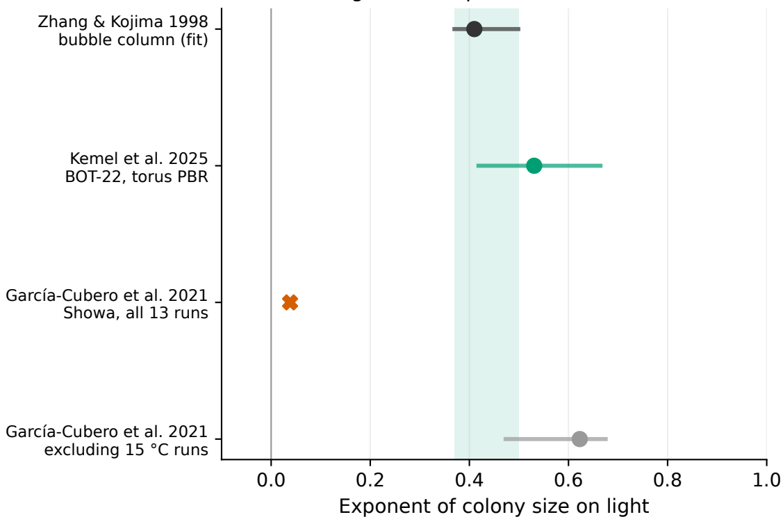
(a) Light-size exponent across studies
