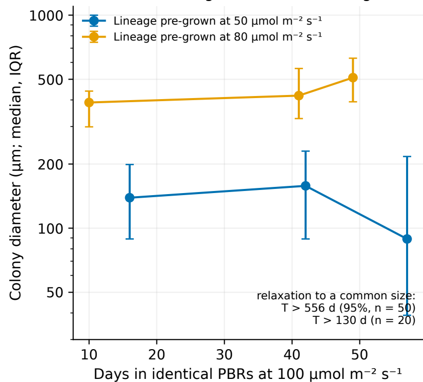
(b) Two lineages under identical light
