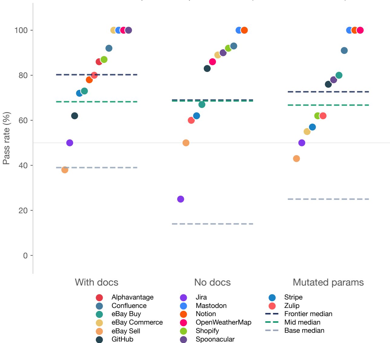
Distribution of pass rates per condition (dashed = tier median)
