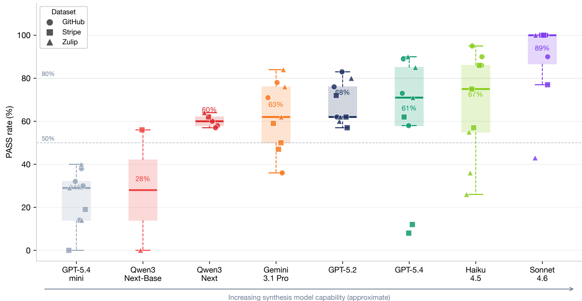
Synthesis model capability vs agent pass rate (GitHub · Stripe · Zulip — common evaluation set)
