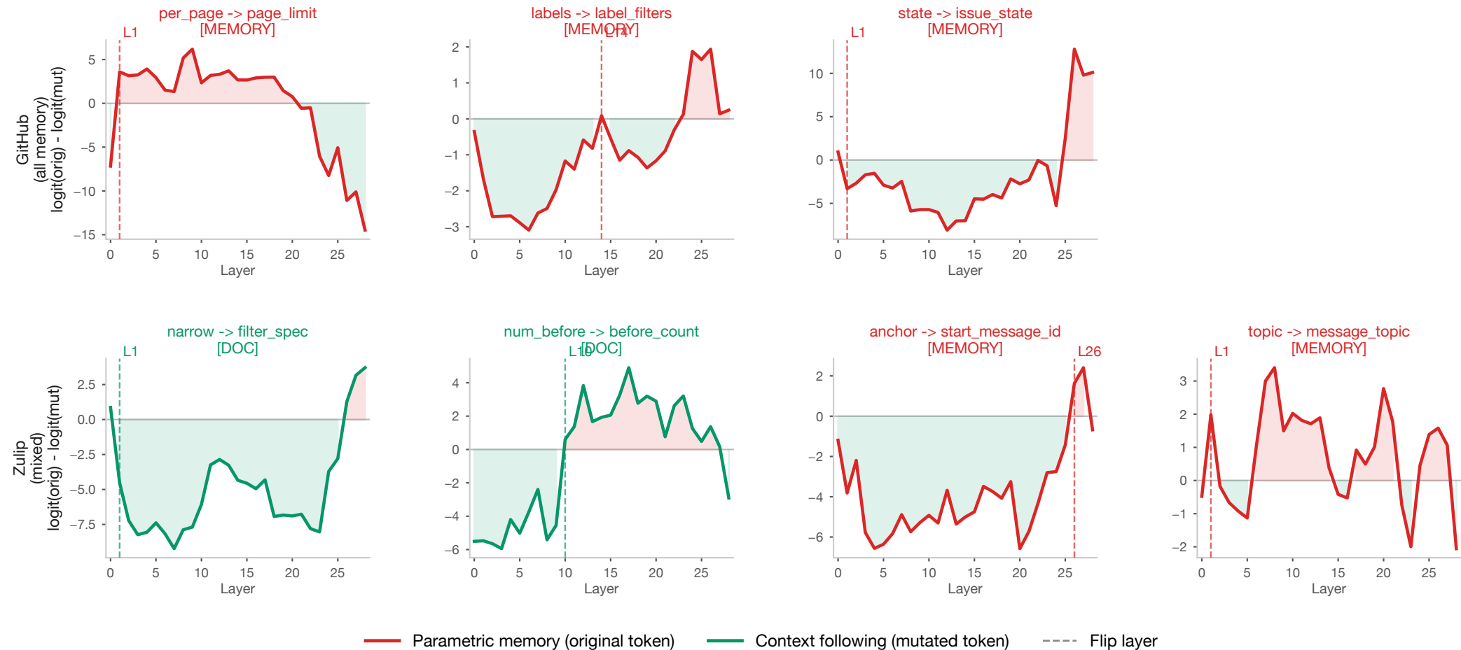
Logit-lens traces: \text{logit}(\text{original}) - \text{logit}(\text{mutated}) per transformer layer Positive = model prefers training-time name; negative = model follows documentation
